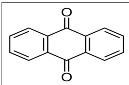
Figure 1. Chemical structure of Anthraquinone
